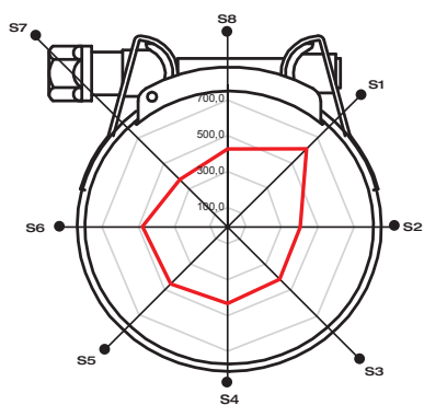
Polar Diagram
